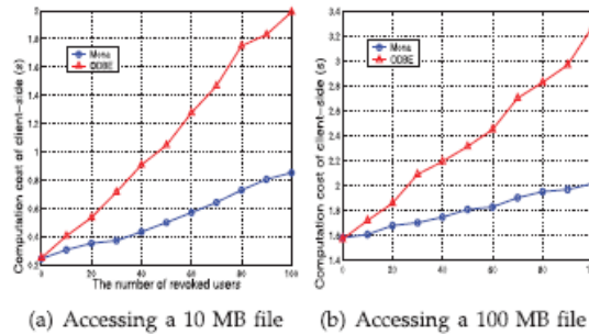
Fig. 3. Comparison on client computation cost for file access between this scheme and ODBE.
