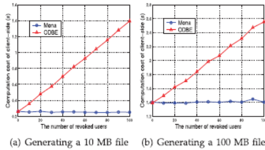
Fig. 2. Comparison on client computation cost for file generation between this scheme and ODBE.
