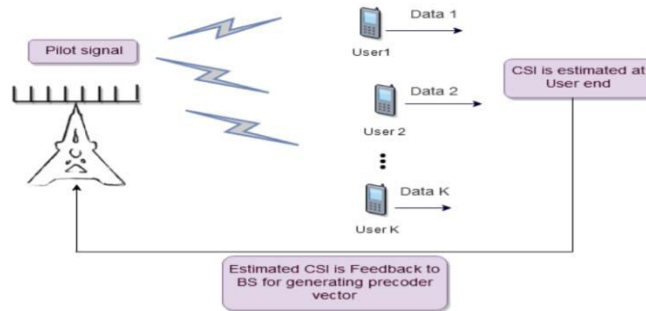
Figure 4: Downlink transmission in an FDD Massive MIMO system
