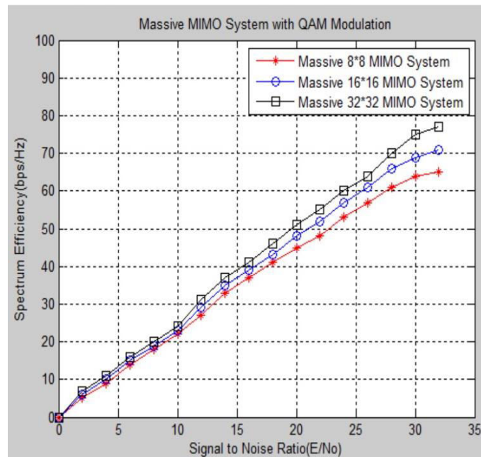
Figure 9: Spectrum Efficiency vs SNR for Cell free Massive 8x8 System with QR-RLS based Channel Estimation Technique
