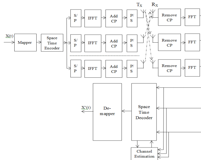
Figure 5: Massive MIMO System Models with Channel Estimation Technique
