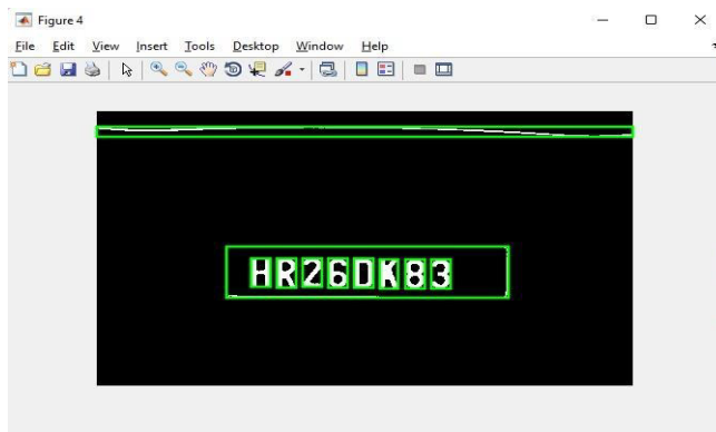
Figure 6: Character Segmentation
